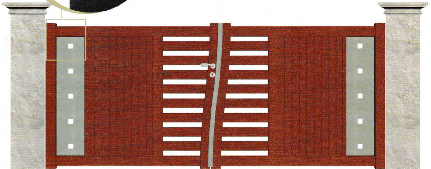
Sculptor
