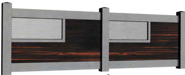
Major
