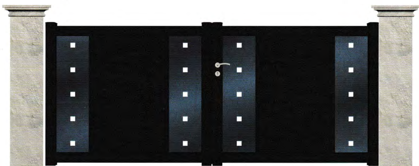
Fornax
